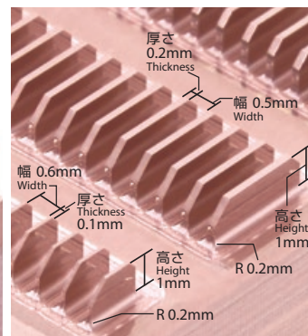
拡大写真 Enlarged Photo
